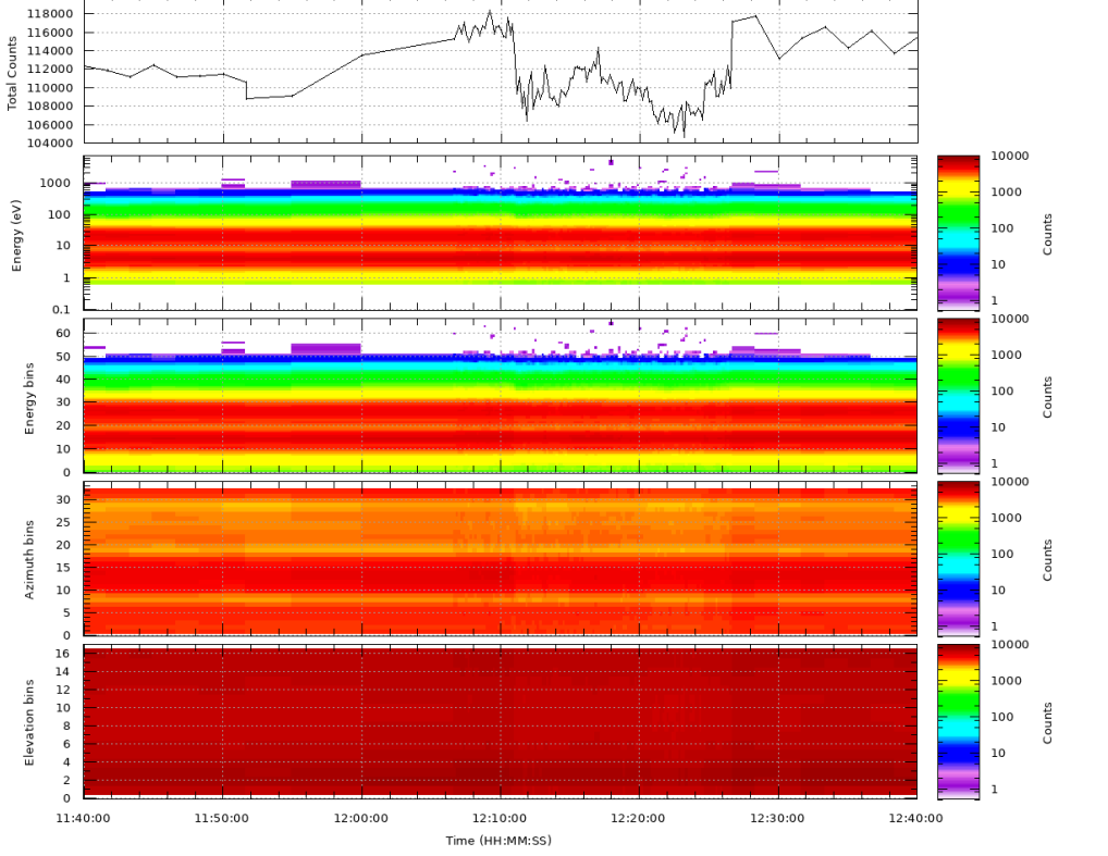
EAS2 Nominal Mode 3D data, counts summed for all other variables, 2020-05-08T11:40:00 - 2020-05-08T12:40:00
