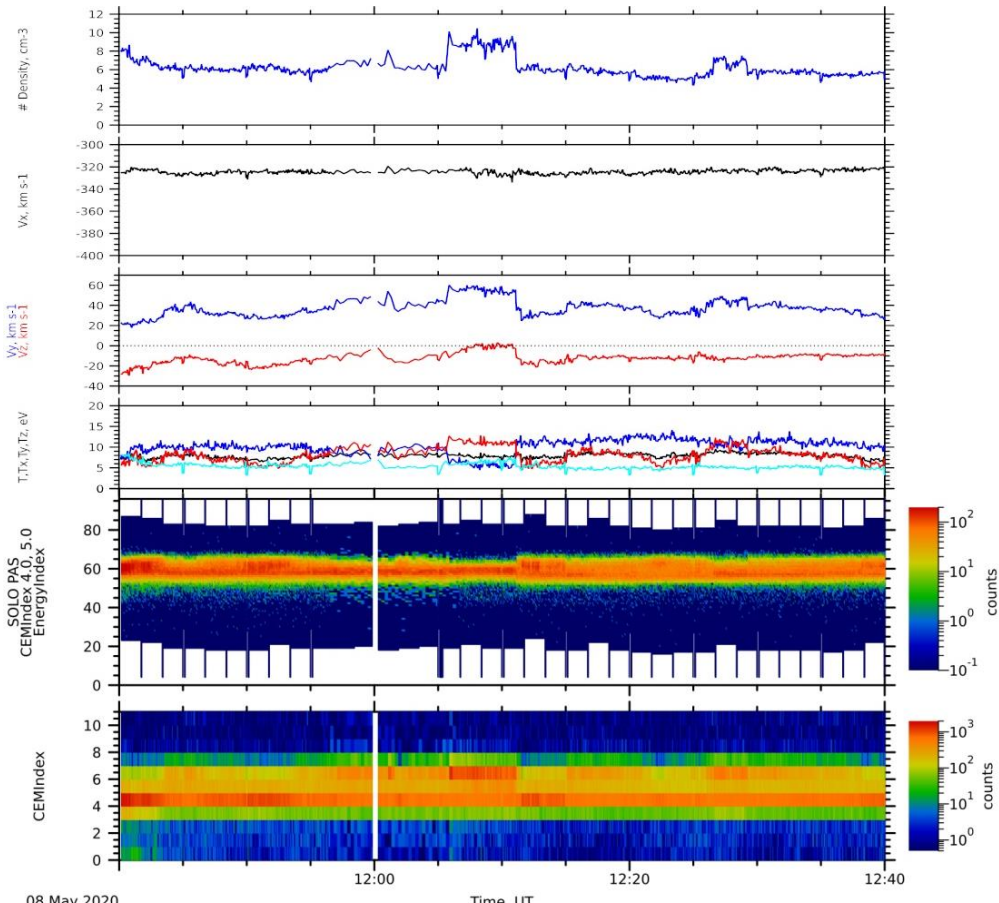
HIS Rates 2020-05-08T114020.065_2020-05-08T123950.025
