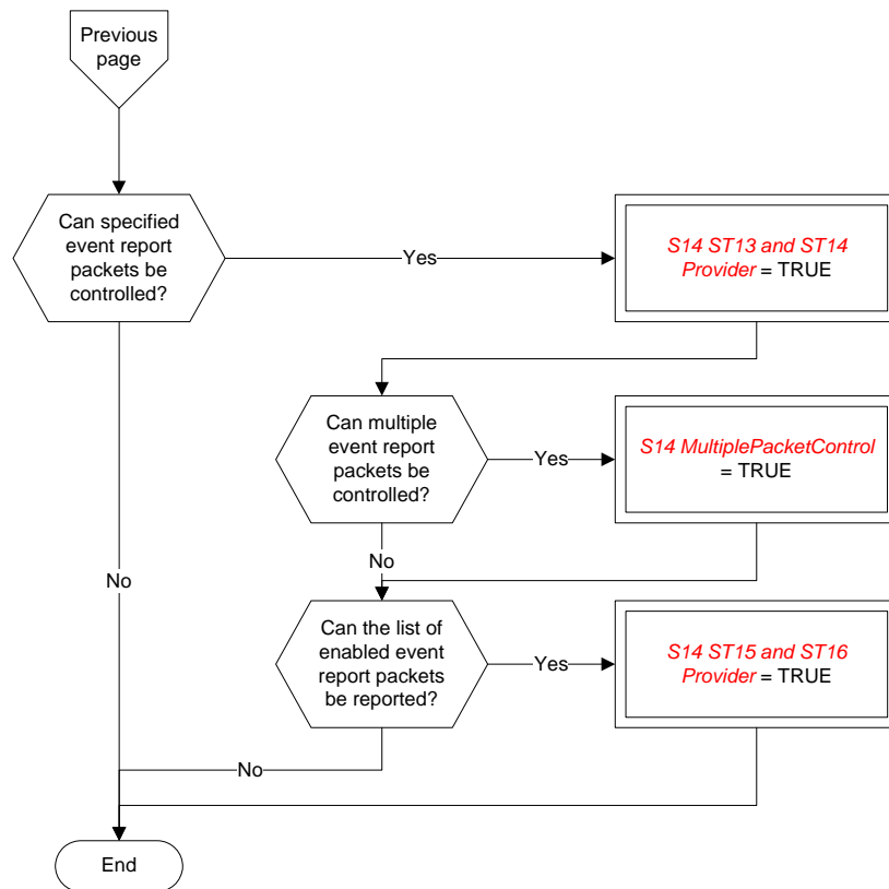
Figure A-13: Tailoring choices for the packet forwarding control service (View 2)
