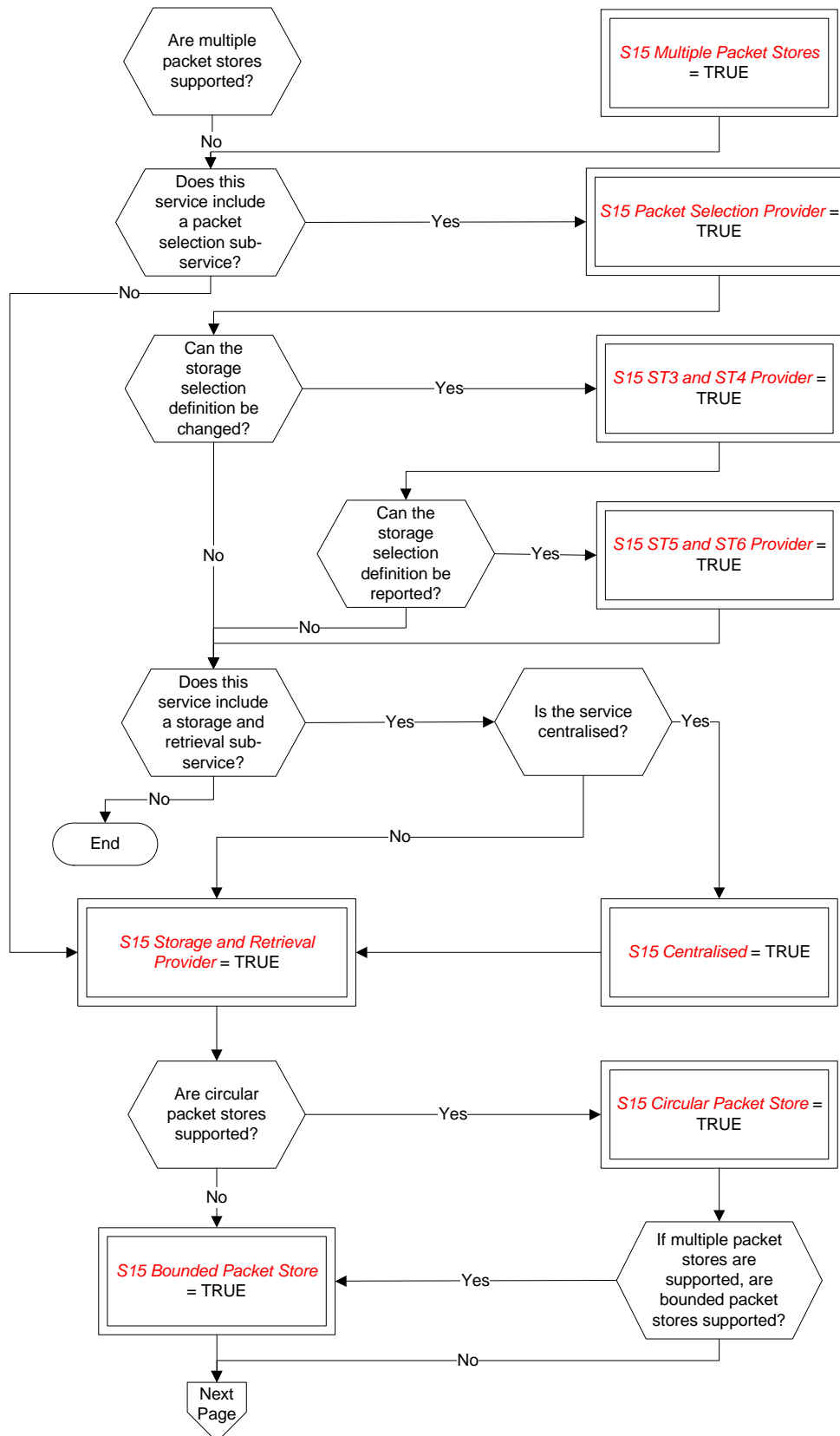
Figure A-14: Tailoring choices for the on-board storage and retrieval service (View 1)
