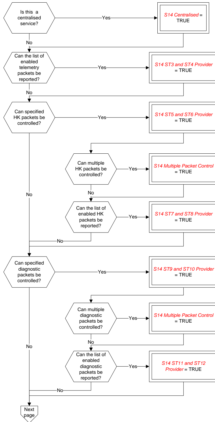
Figure A-13: Tailoring choices for the packet forwarding control service (View 1)
