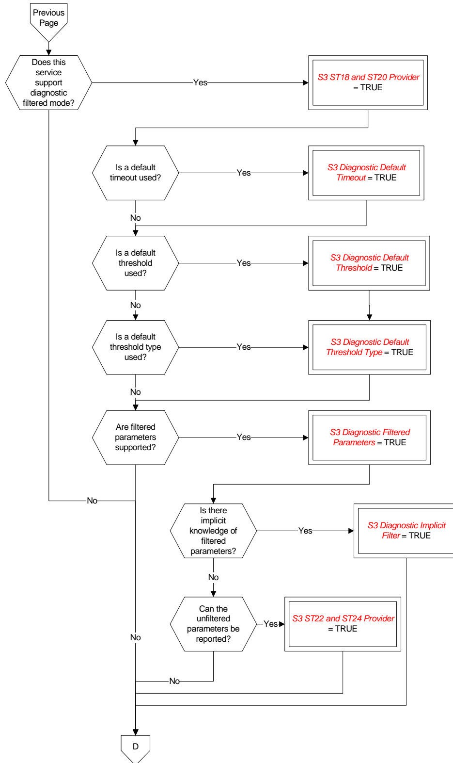
Figure A-4: Tailoring choices for the housekeeping and diagnostic data reporting service (View 5)
