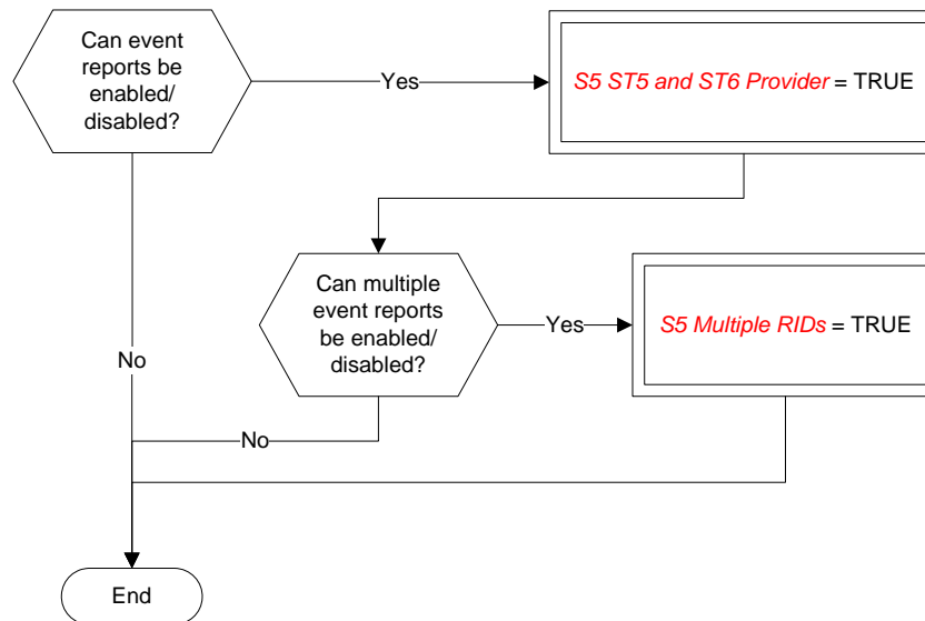
Figure A-6: Tailoring choices for the event reporting service
