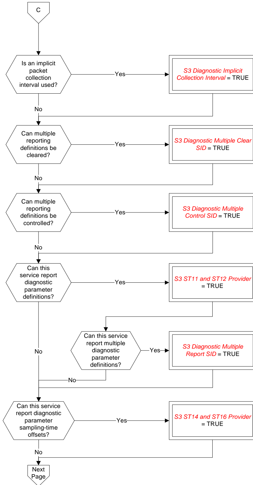
Figure A-4: Tailoring choices for the housekeeping and diagnostic data reporting service (View 4)
