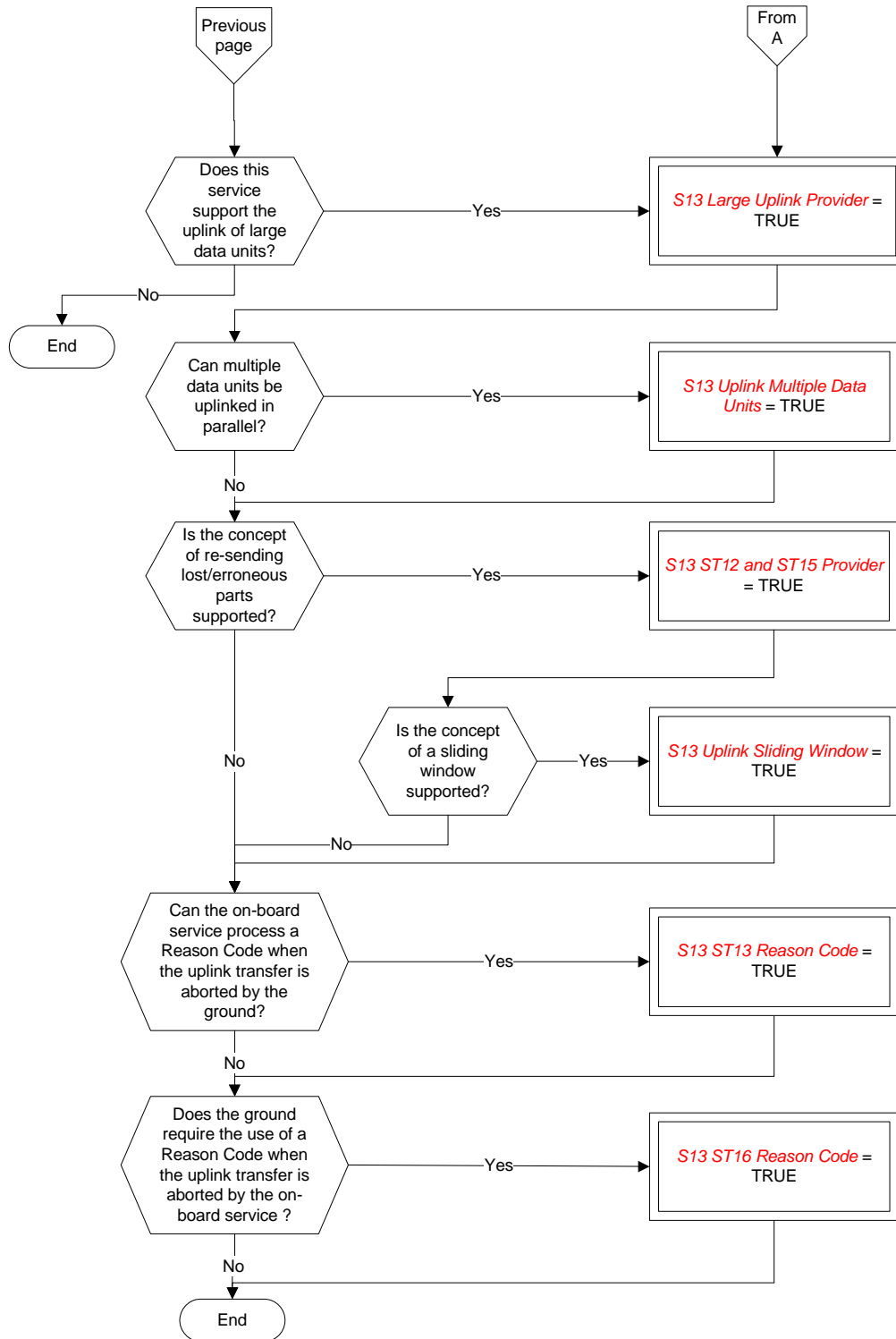
Figure A-12: Tailoring choices for the large data transfer service (View 2)
