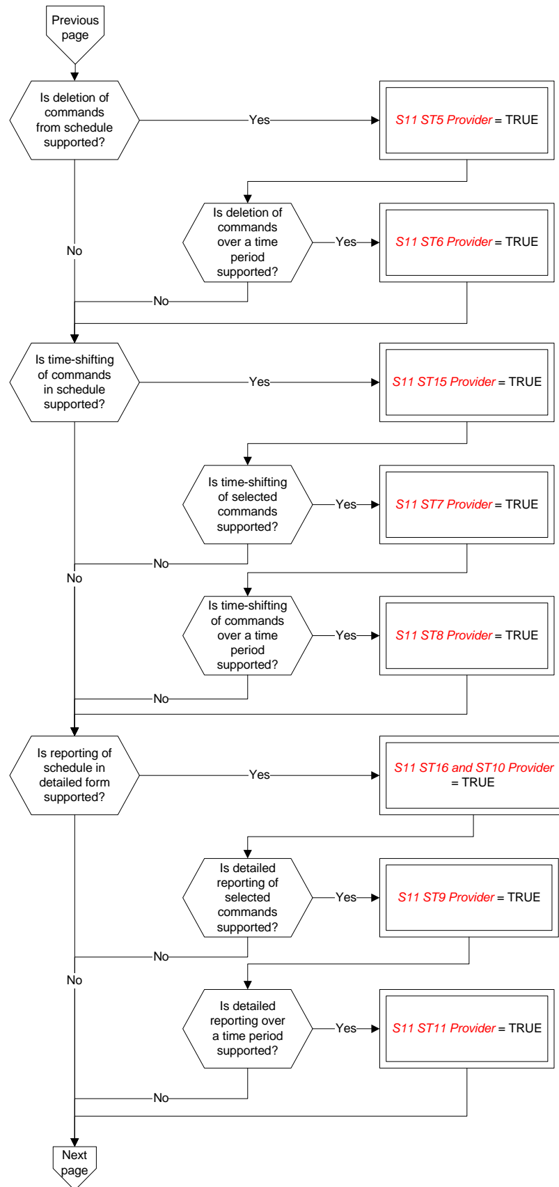
Figure A-10: Tailoring choices for the on-board operations scheduling service (View 2)
