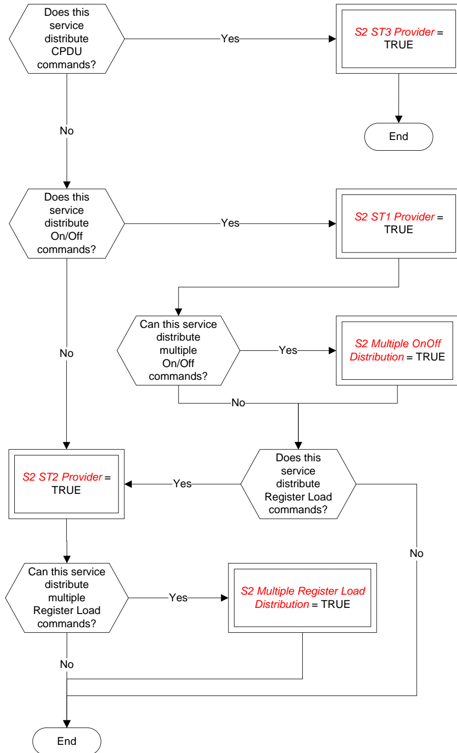
Figure A-3: Tailoring choices for the device command distribution service
