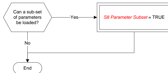
Figure A-8: Tailoring choices for the function management service
