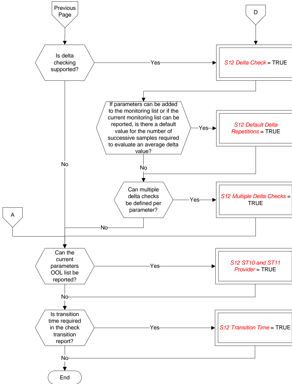
Figure A-11: Tailoring choices for the on-board monitoring service (View 3)
