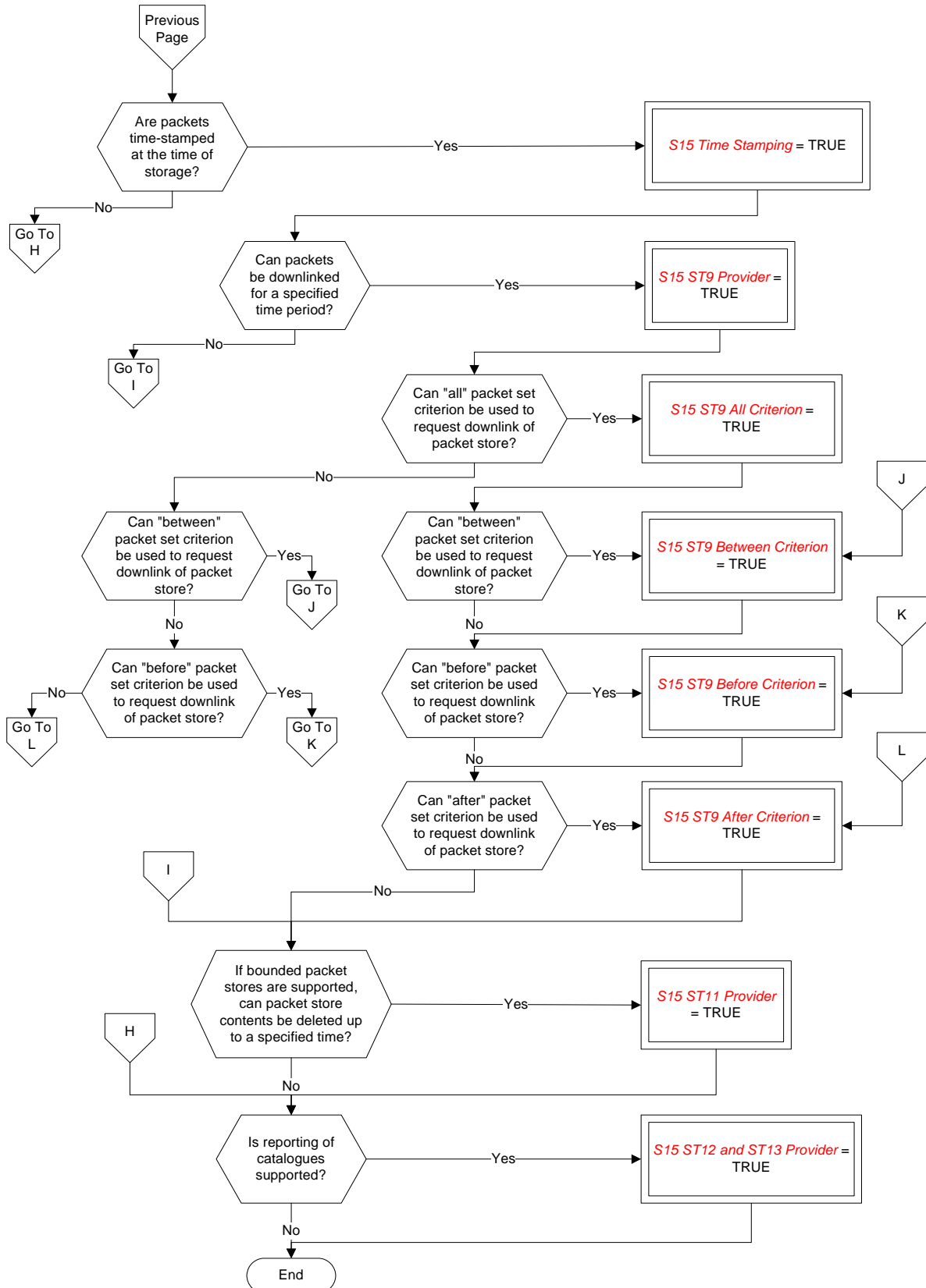
Figure A-14: Tailoring choices for the on-board storage and retrieval service (View 3)
