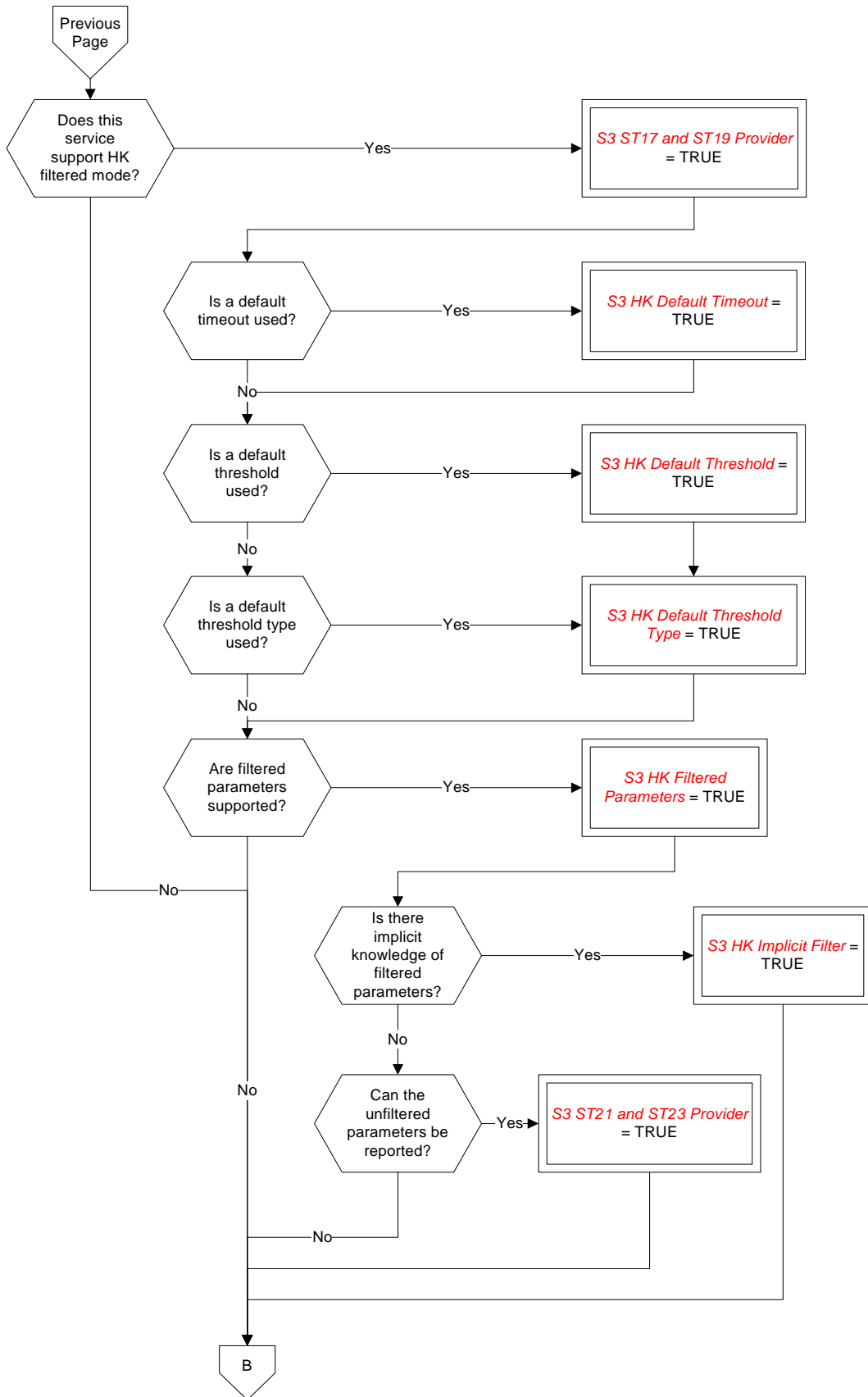
Figure A-4: Tailoring choices for the housekeeping and diagnostic data reporting service (View 3)
