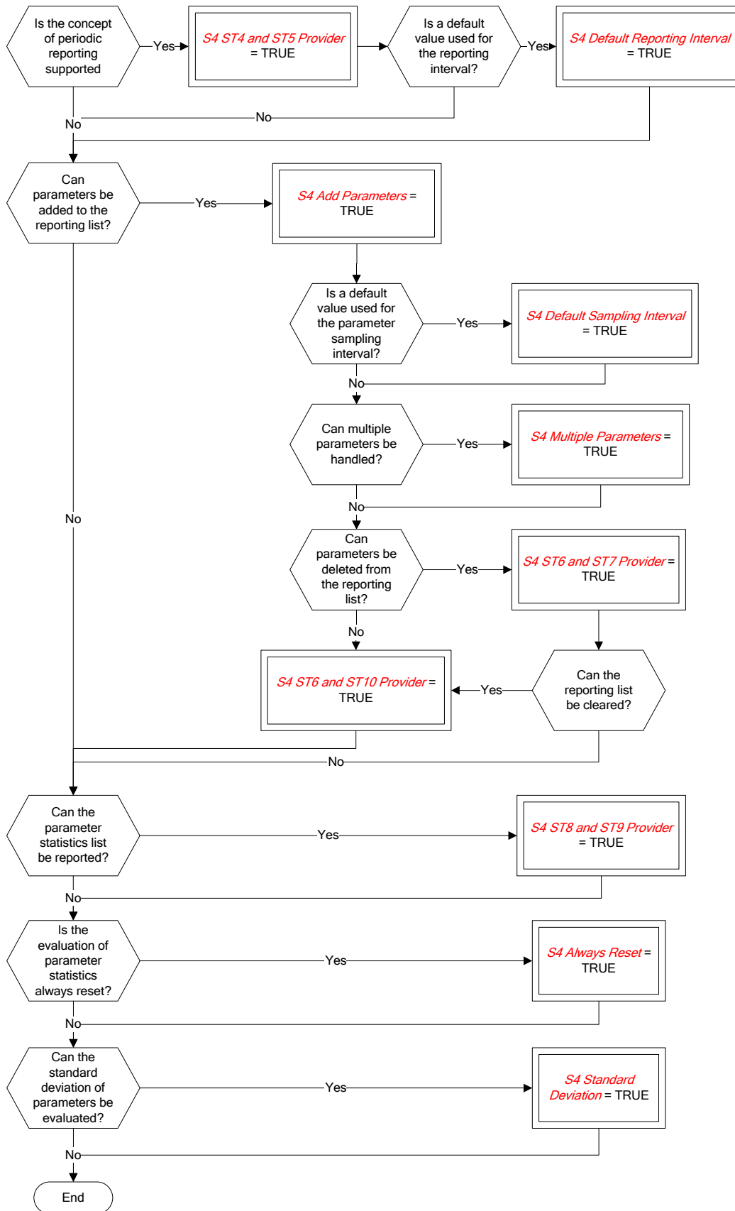
Figure A-5 Tailoring choices for the parameter statistics reporting service
