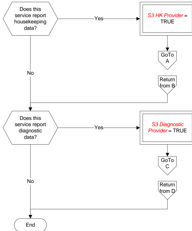
Figure A-4: Tailoring choices for the housekeeping and diagnostic data reporting service (View 1)
