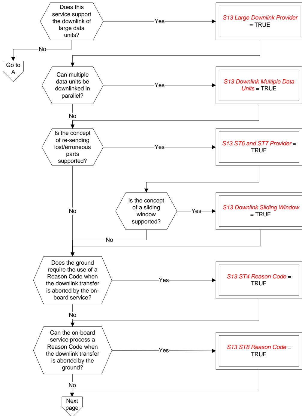
Figure A-12: Tailoring choices for the large data transfer service (View 1)
