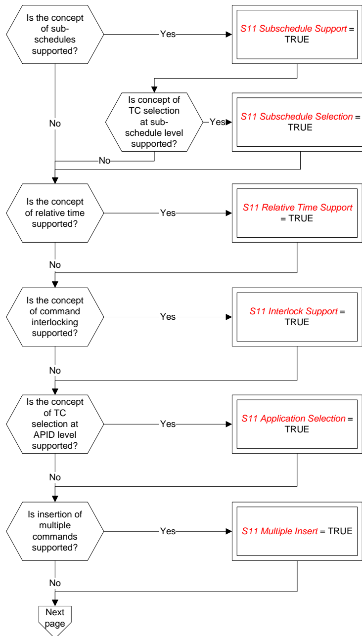
Figure A-10: Tailoring choices for the on-board operations scheduling service (View 1)
