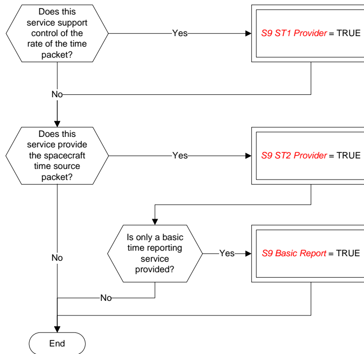
Figure A-9: Tailoring choices for the time management service
