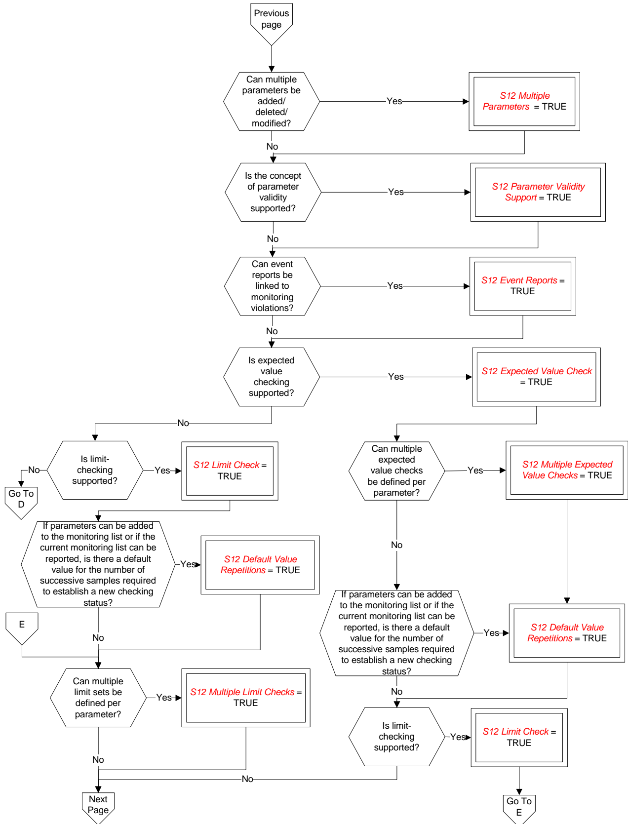
Figure A-11: Tailoring choices for the on-board monitoring service (View 2)
