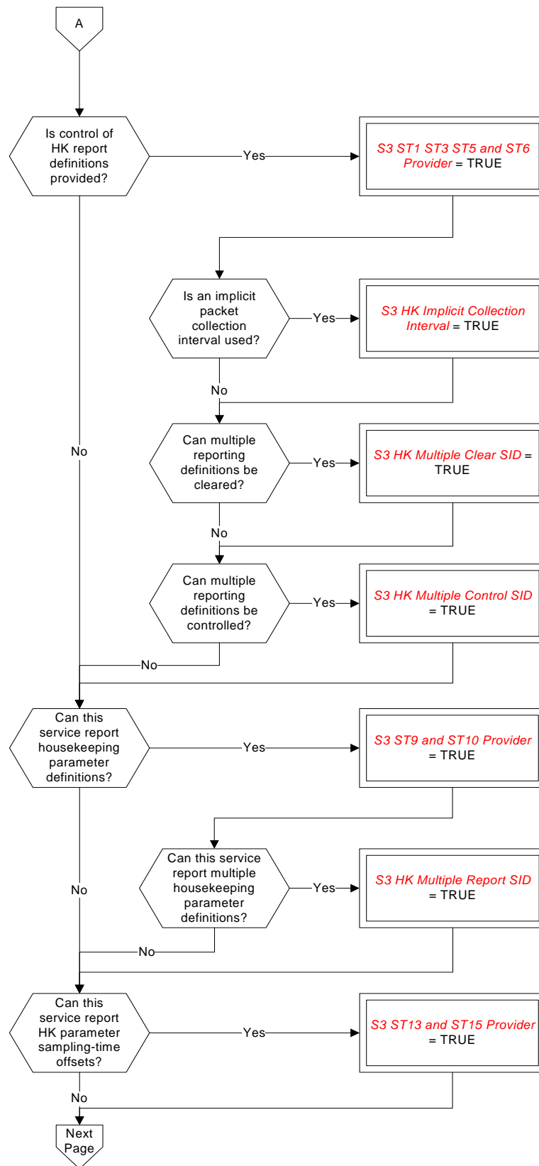
Figure A-4: Tailoring choices for the housekeeping and diagnostic data reporting service (View 2)
