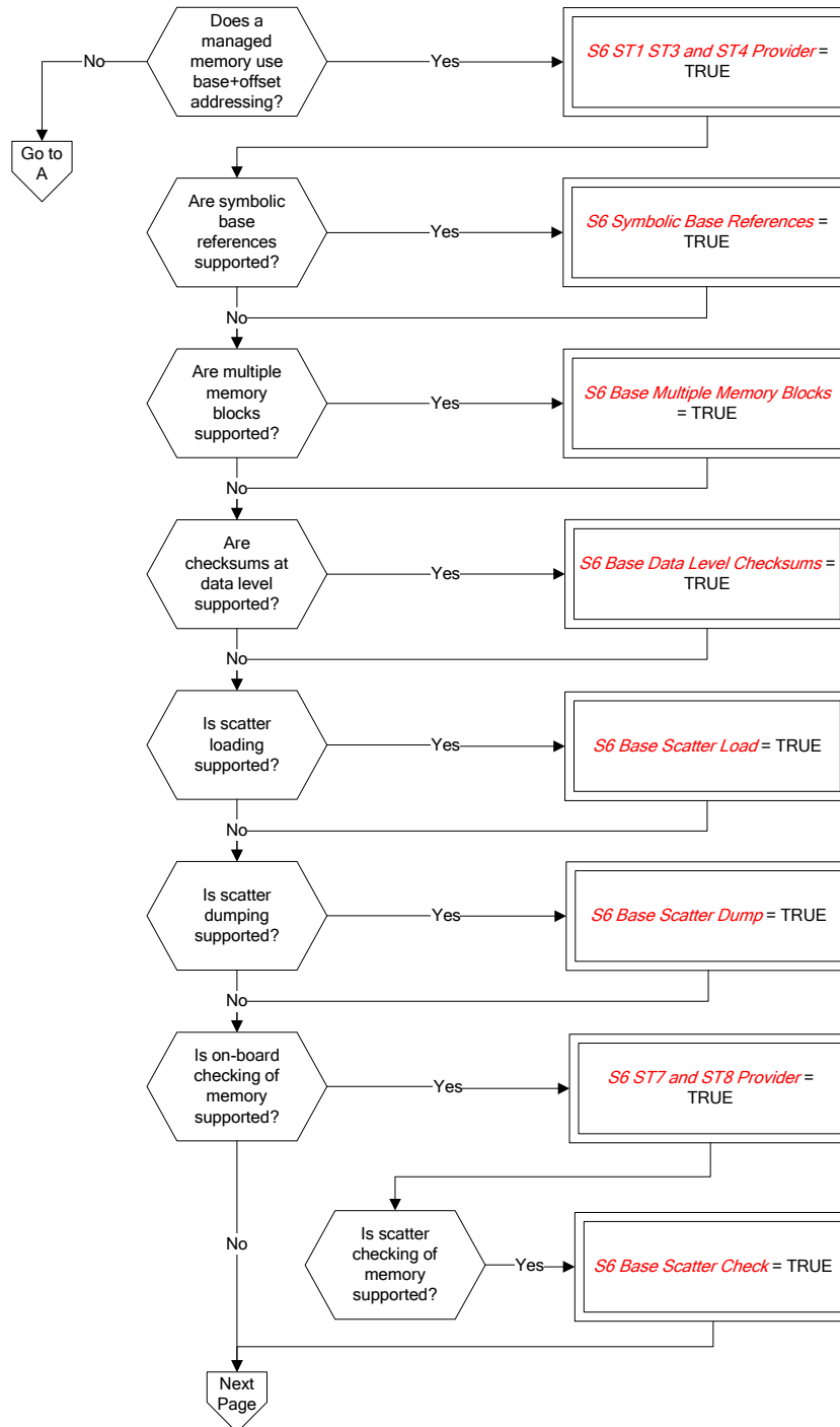
Figure A-7: Tailoring choices for the memory management service (View 1)
