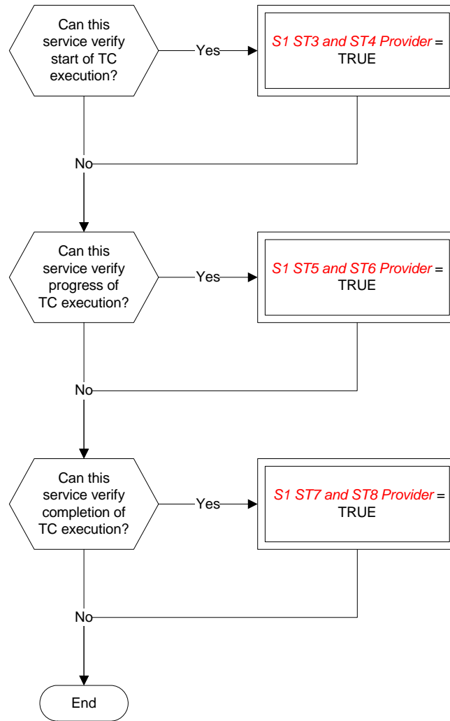
Figure A-2: Tailoring choices for the telecommand verification service
