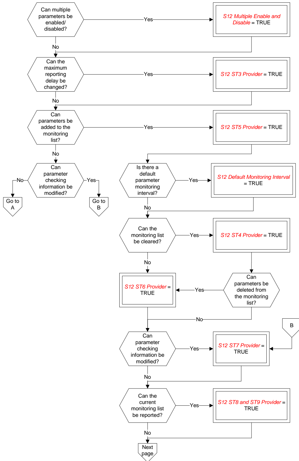
Figure A-11: Tailoring choices for the on-board monitoring service (View 1)
