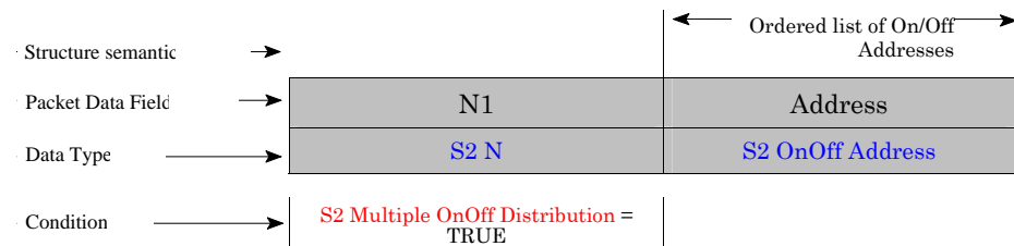
Figure A-1: Diagram convention for PUS packet structures
