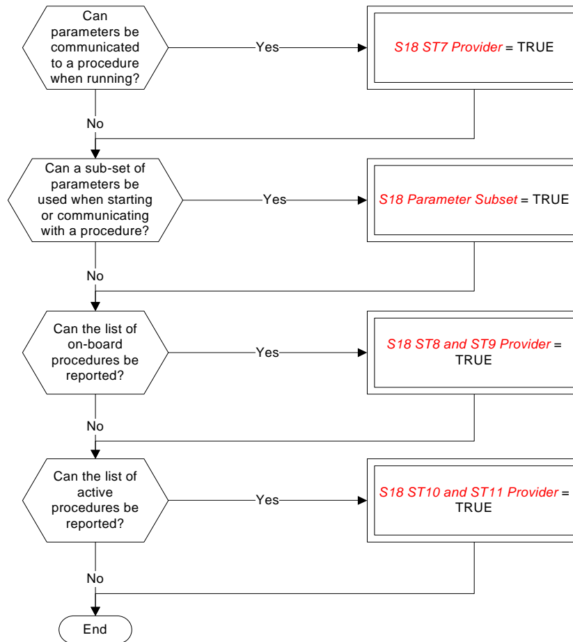
Figure A-15: Tailoring choices for the on-board operations procedure service
