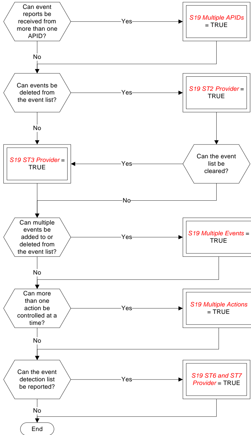
Figure A-16 Tailoring choices for the event/action service
