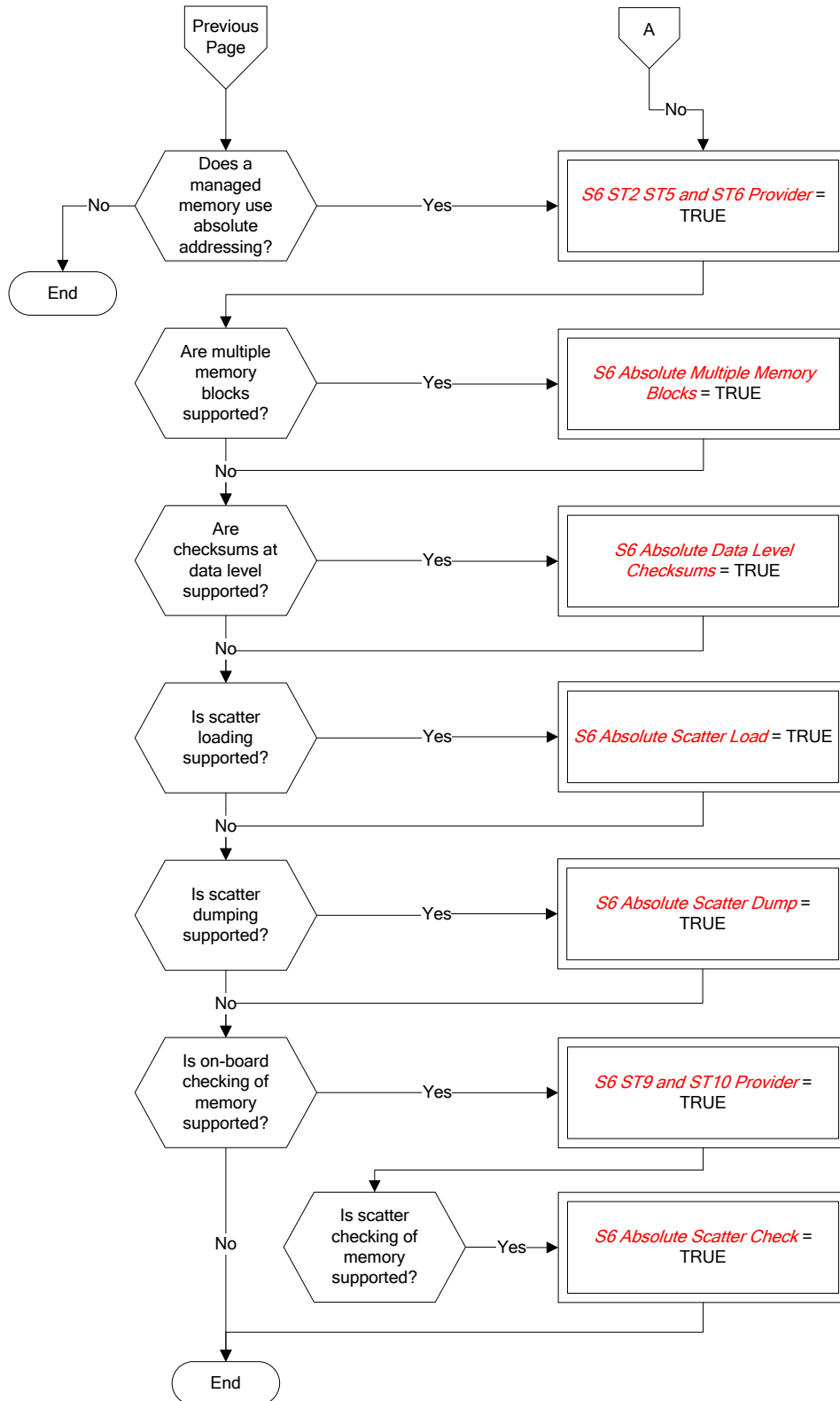
Figure A-7: Tailoring choices for the memory management service (View 2)
