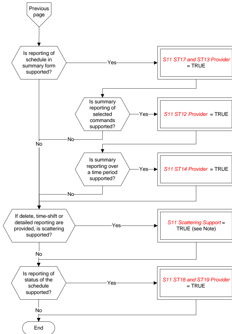
Figure A-10: Tailoring choices for the on-board operations scheduling service (View 3)
