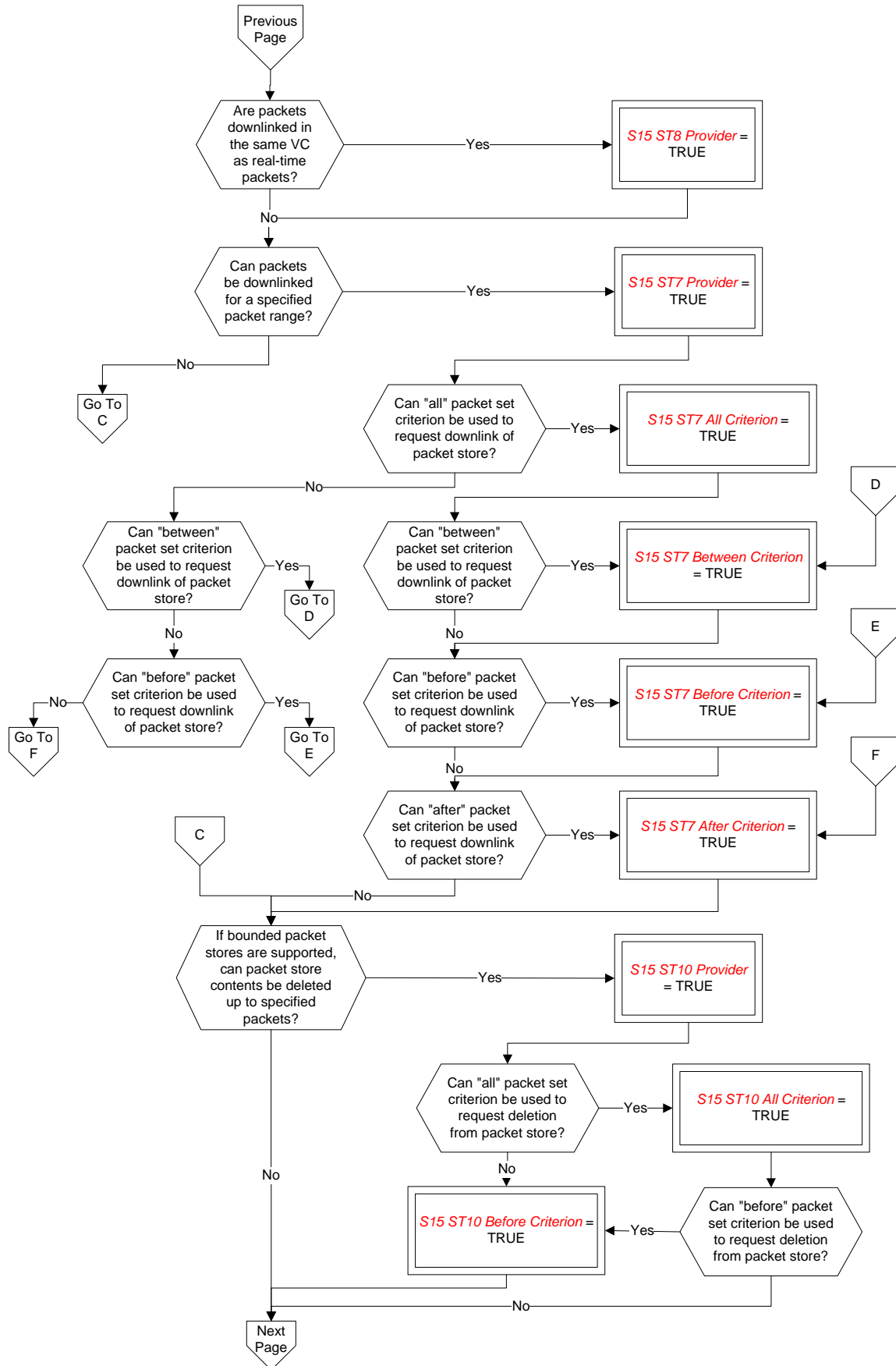
Figure A-14: Tailoring choices for the on-board storage and retrieval service (View 2)
