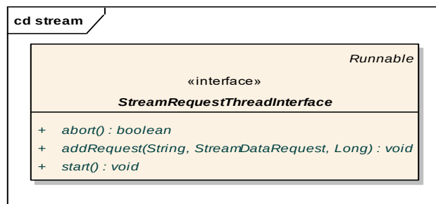
Figure 19 - Stream Request Interface
