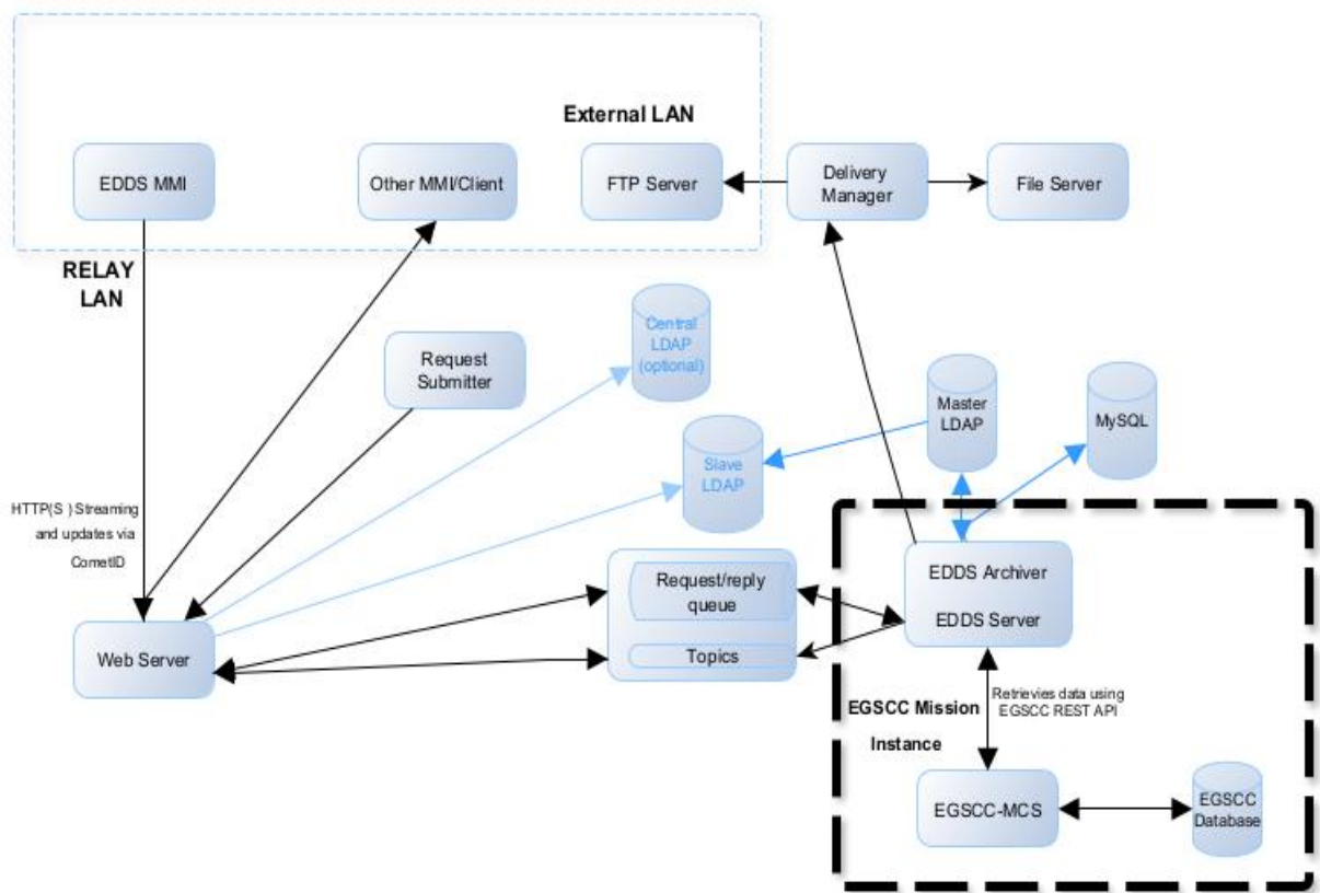
Figure 42 - EDDS-CC Top level component architecture
