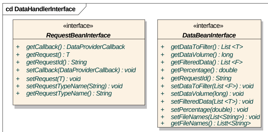
Figure 21 - Request and Data Bean Interfaces
