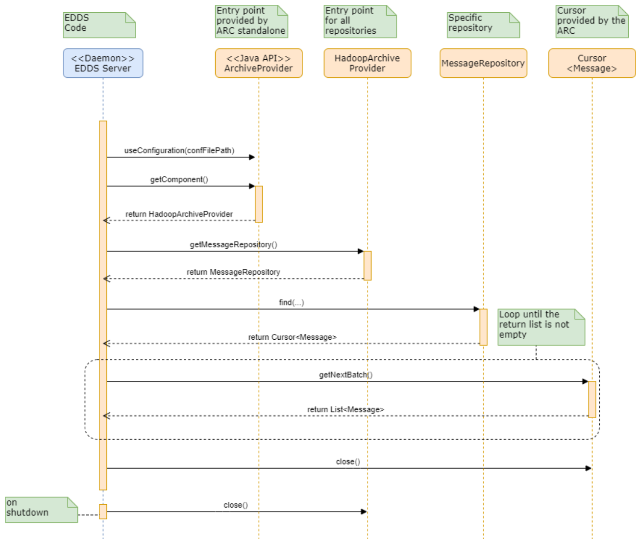
Figure 456 - Sequence diagram to get Message data
