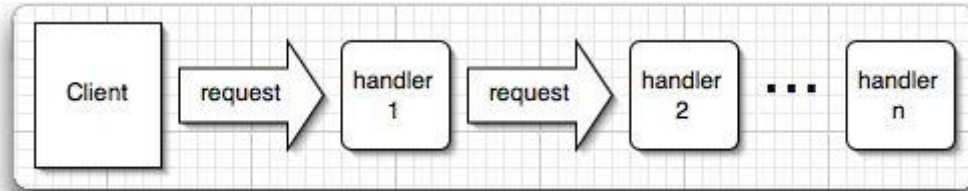
Figure 434 - CoR Pattern
