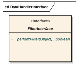
Figure 22 - Filter Interface
