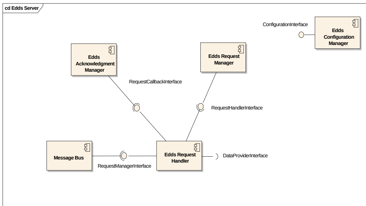
Figure 17 - EDDS Server
