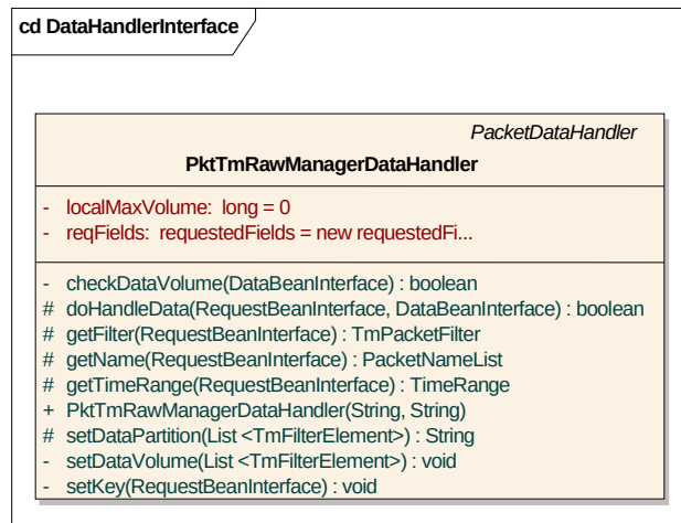
Figure 27 - TmPacket Handlers
