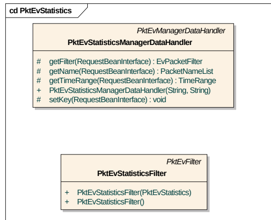
Figure 34 - Ev Packet Statistics Handlers
