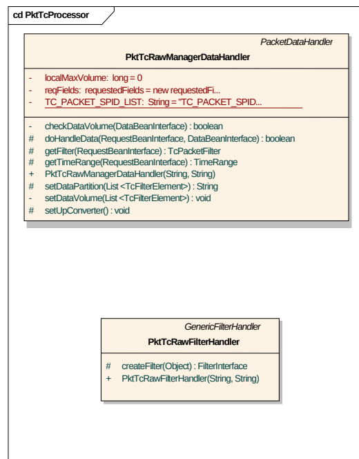
Figure 30 - Tc Packet Raw Handlers
