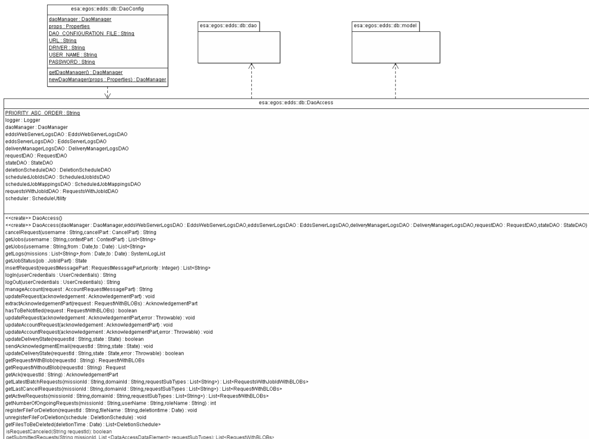
Figure 423 - database facade
