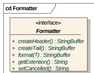
Figure 23 - Formatter interface
