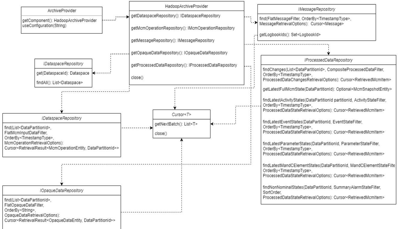
Figure 445 - ARC Standalone API partial class diagram
