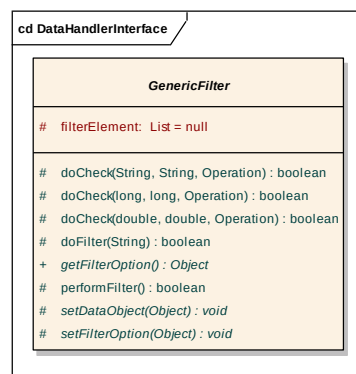
Figure 25 - Generic Filter Class
