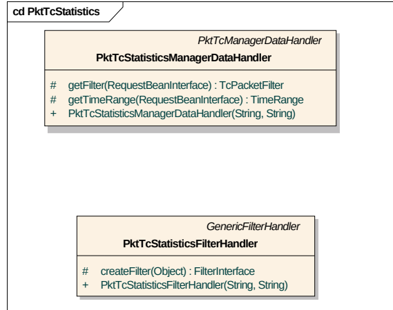
Figure 31 - Tc Packet Statistics Handlers
