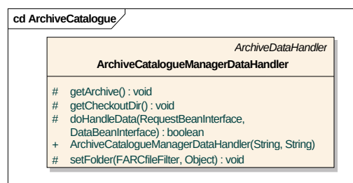
Figure 36 - Archive Catalogue Manager Data Handler
