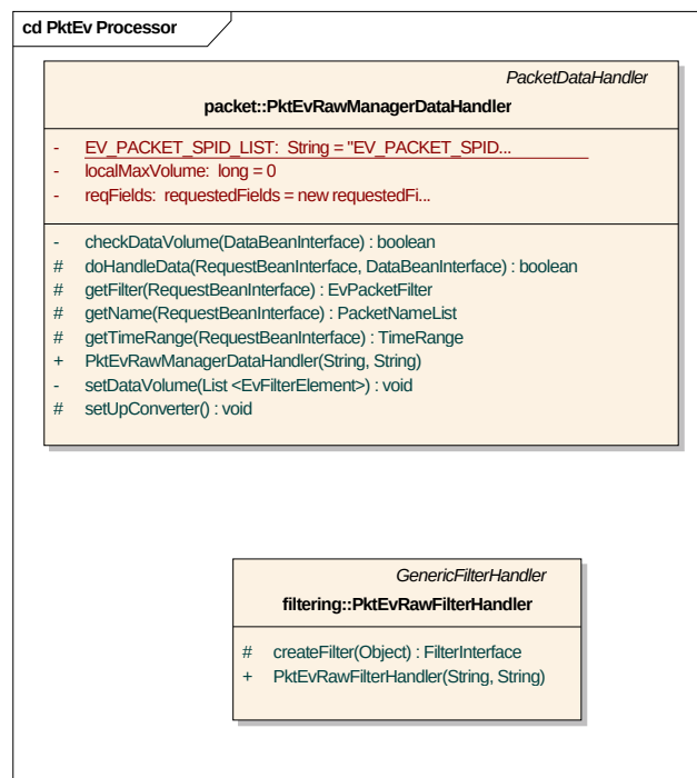
Figure 33 - Ev Packet Handlers
