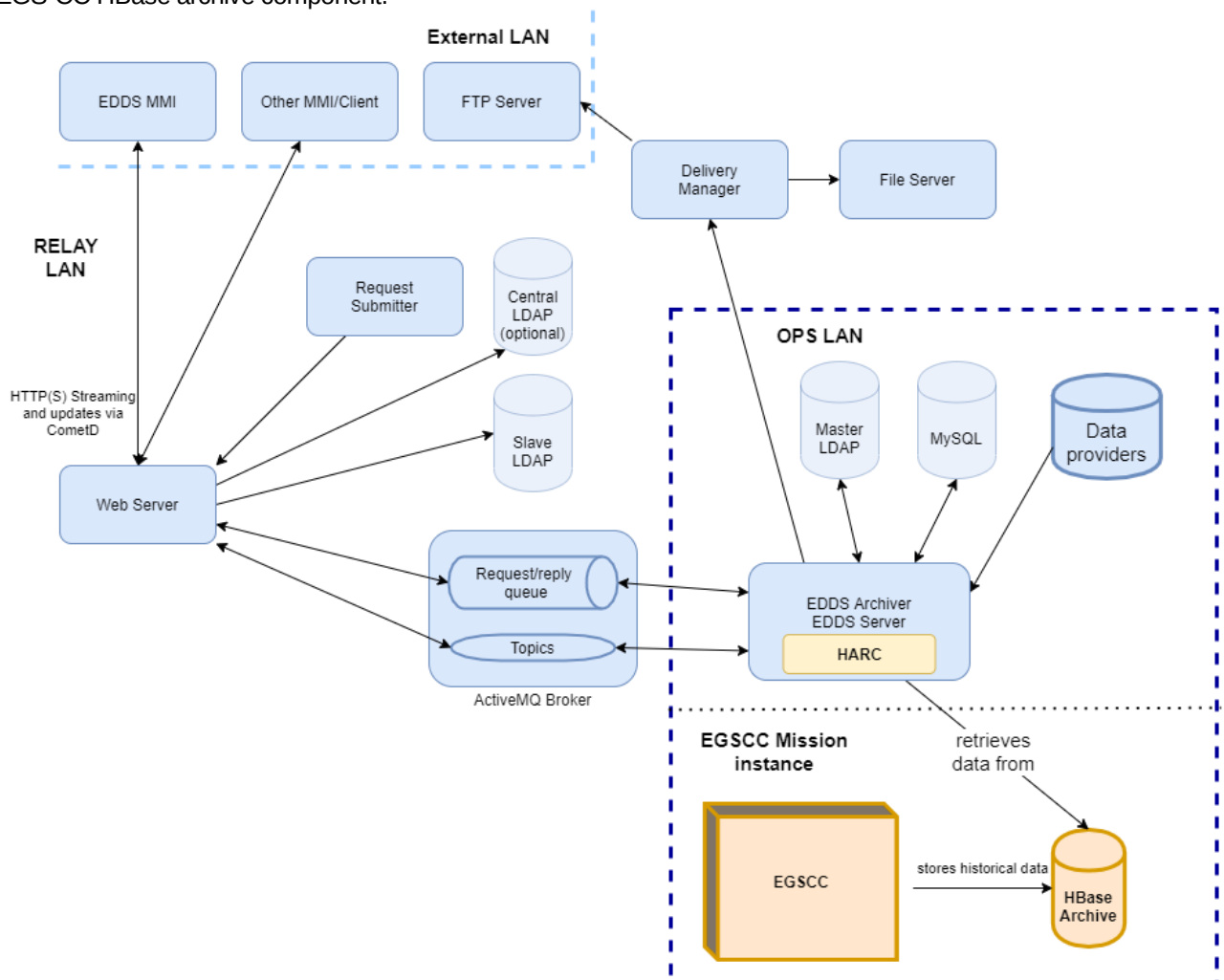
Figure 40 - EDDS-CC Top level component architecture
