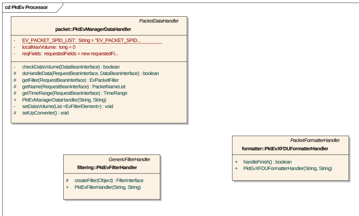
Figure 32 - Ev Packet Handlers
