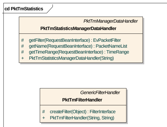
Figure 28 - TM Packet Statistics Handlers
