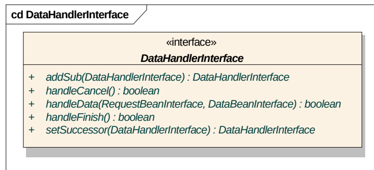
Figure 20 - Data Handler Interface
