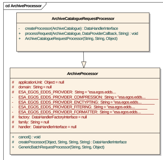
Figure 35 - ArchiveCatalogueRequestProcessor
