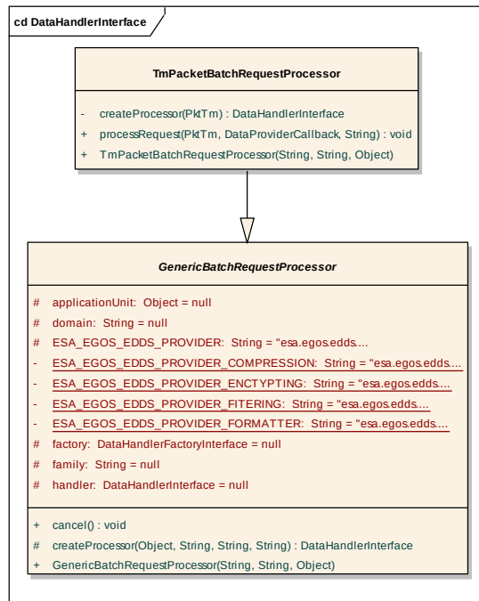
Figure 26 - TmPacketBatchRequestProcessor
