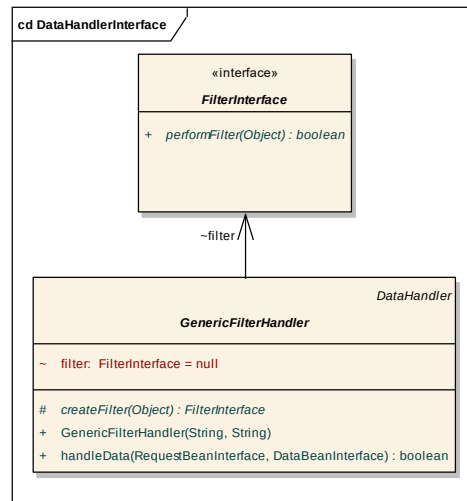
Figure 24 - Generic Filter Handler
