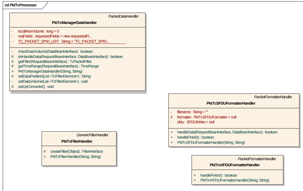
Figure 29 - Tc Packet Handlers
